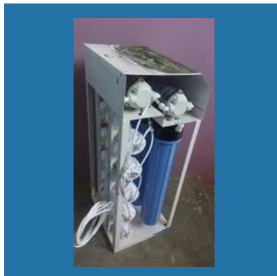
Covered RO System
